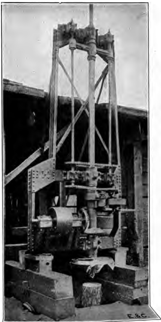
Fig. 58. Rotary Stump Cutting Machine
